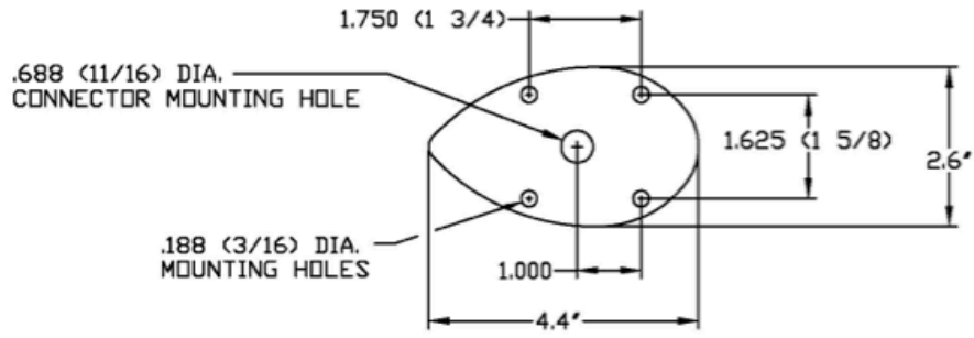
MOUNTING INFORMATION
